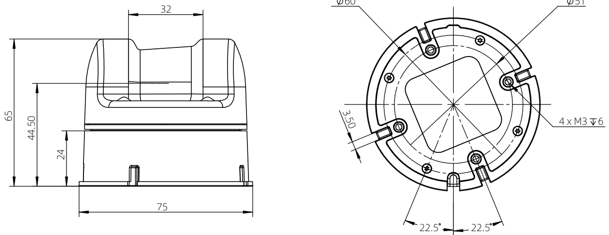
L2 Mechanical Dimensions
